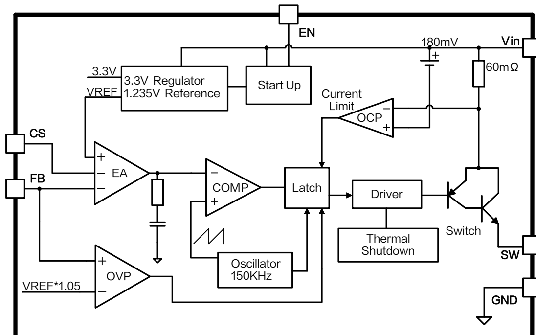
Figure3. Function Block Diagram of XL4001
